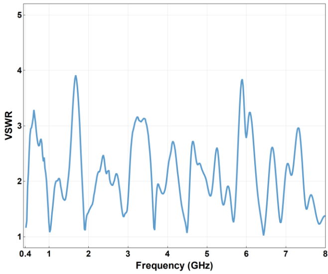
HOA-80 驻波比
