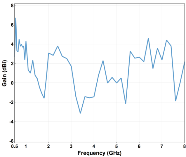
HOA-80 增益
